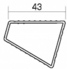
●踏ざん形状
